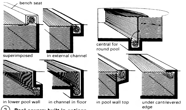
② Pool covers: built-in options
